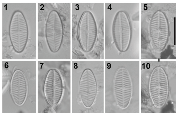
Figures 1–10. Platessa deqinensis sp. nov., LM, DIC. Valve views, showing size range and variability of the holotype population. (1–5) Raphe valves. Figure 1 is the holotype. (6–10) Rapheless valves. Scale bar 10 \mu\text{m} .
