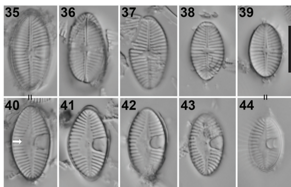
Figures 35–44. Achnanthes joursacense Héribaude 1903. Slide1 (The specimens were provided by Prof. Kociolek, J.P.). LM, DIC. Valve views. (35–39) Raphe valves. (40–44) Rapheless valves. White arrow in Fig 40 shows the axial area expanded in central area. Scale bar 10 \mu m.
