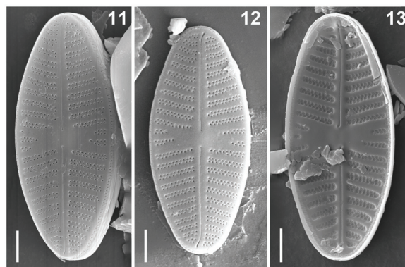
Figures 11–13. Platessa deqinensis sp. nov., SEM, raphe valve views. (11–12) External view of the raphe valves. (13) Internal view of the raphe valve. Scale bars 2 \mu\text{m} .
