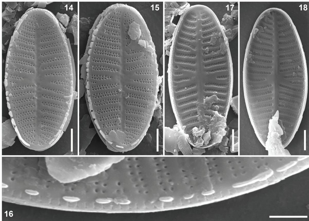
Figures 14–18. Platessa deqinensis sp. nov., SEM, rapheless views. (14–15) External view of the raphe valves. (16) Detail of valve showing the short and wide spine-like projections on the margin. (17–18) Internal view of the rapheless valves. Scale bars 2 \mu\text{m} (14–15, 17–18) and 1 \mu\text{m} (16).
