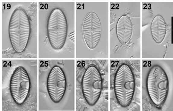
Figures 19–28. Planoplattessa joursacense . LM, DIC. Valve views. (19–23) Raphe valves. (24–28) Rapheless valves. Scale bar 10 µm.
