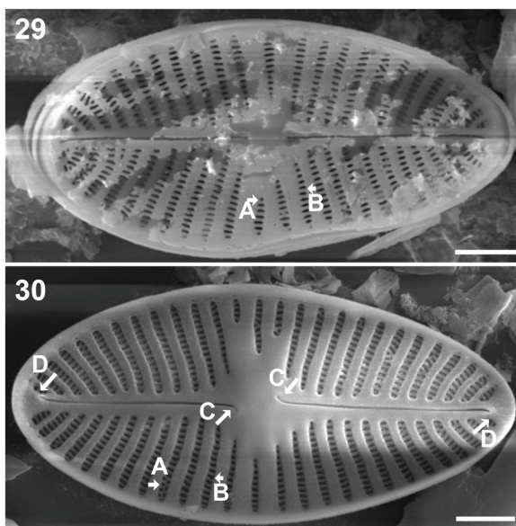
Figures 29–30. Planoplattessa joursacense . SEM, raphe valve views. (29) External view of the raphe valve. Arrows A and B show the round and slit-like shape of the areolae, respectively. (30) Internal view of the raphe valve. Arrows A and B same as mentioned previously. Arrows C show the deflected in proximal raphe endings; Arrows D show the helictoglossa. Scale bars 2 µm.
