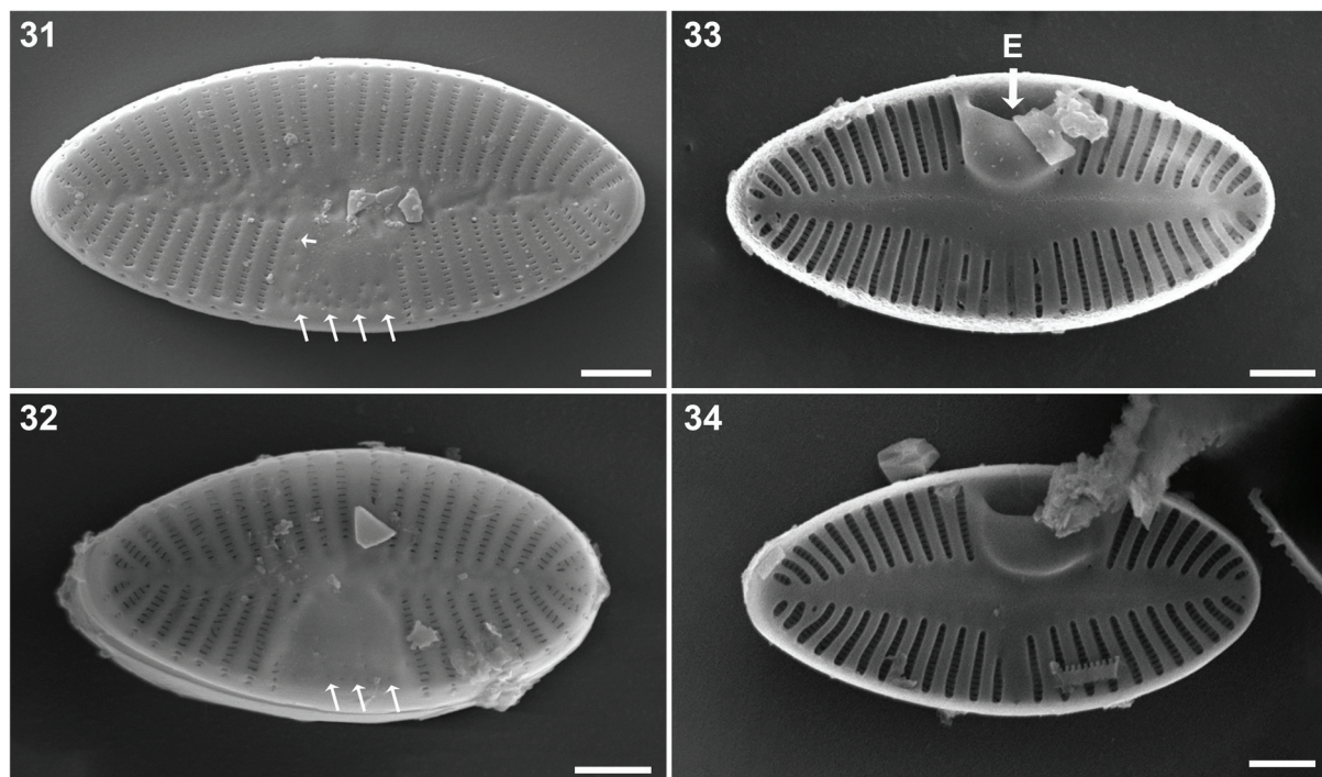
Figures 31–34. Planoplatessa joursacense . SEM, rapheless views. (31–32) External view of the rapheless valves. White arrows show the central area with irregularly arranged fine dots. (33–34) Internal view of the rapheless valves. Arrow E shows the cavum. Scale bars 2 \mu m.
