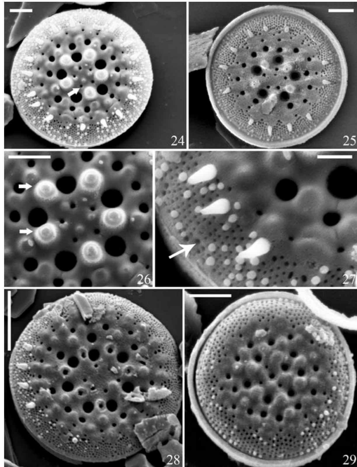
Figs 24–29. Tertiarius juriljii , SEM external valve views, type material: (24) valve view, showing the external openings of the valve face fultoportula (arrow), (25) view of the whole valve, (26) detailed view of the valve centre, showing the distinct valve large granules (white arrows), (27) girdle view showing the spines and the external opening of the fultoportula (white arrow), (28, 29) valve views. Scale bars 5 \mu m (24–26, 29), 2 \mu m (24–26, 29), 1 \mu m (27).
