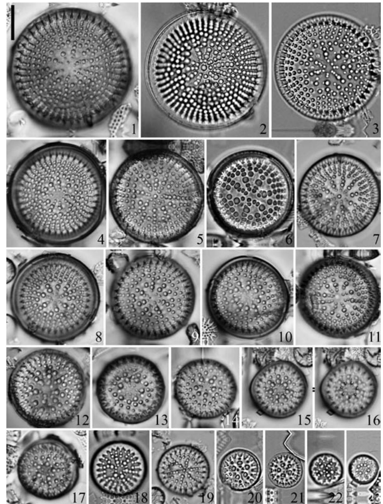
Figs 1–23. Tertiarius juriljii , LM valve views, Mariovo, Macedonia: (1–23): diminution series, (3): Holotype specimen. Scale bar 10 µm.
