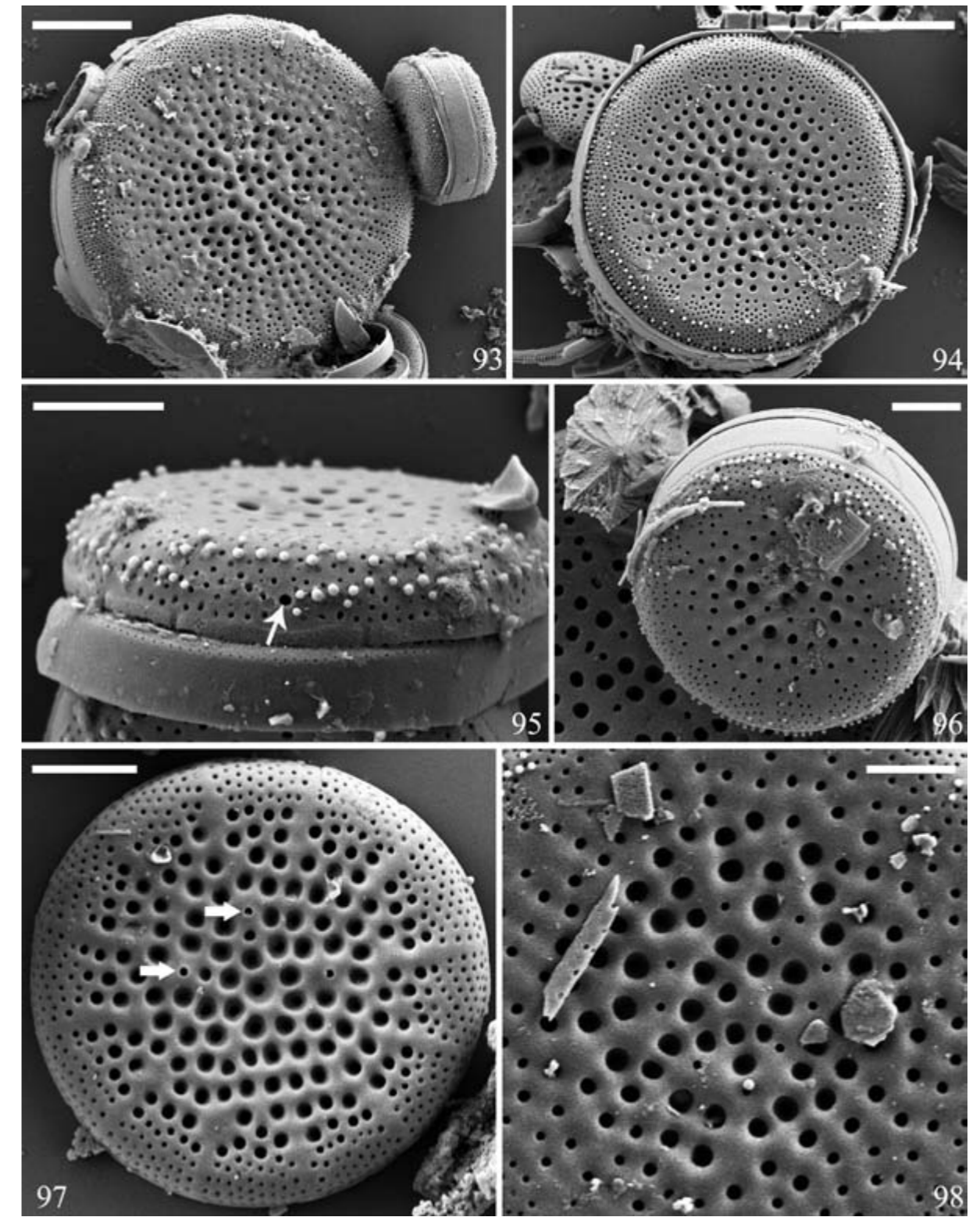
Figs 93–98. Tertiarius mariovensis , SEM external valve views: (93, 94) view of the whole valve, (95) girdle view showing the external opening of the fuloportula (white arrow), (96) view of the whole frustule, (97) close view of the external openings of the valve face fuloportula in corroded specimen (white arrows), (98) detailed view of the central part of the valve in corroded specimen. Scale bar 5 \mu\text{m} (93, 94), 2 \mu\text{m} (95–98).
