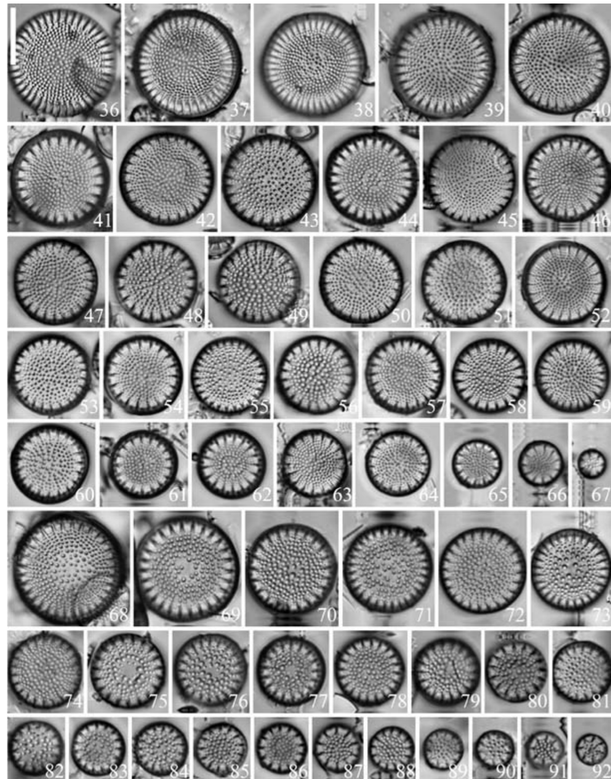
Figs 36–92. Tertiarius mariovensis , LM valve views, Mariovo, Macedonia, diminution series. Scale bar 10 \mu\text{m} .
